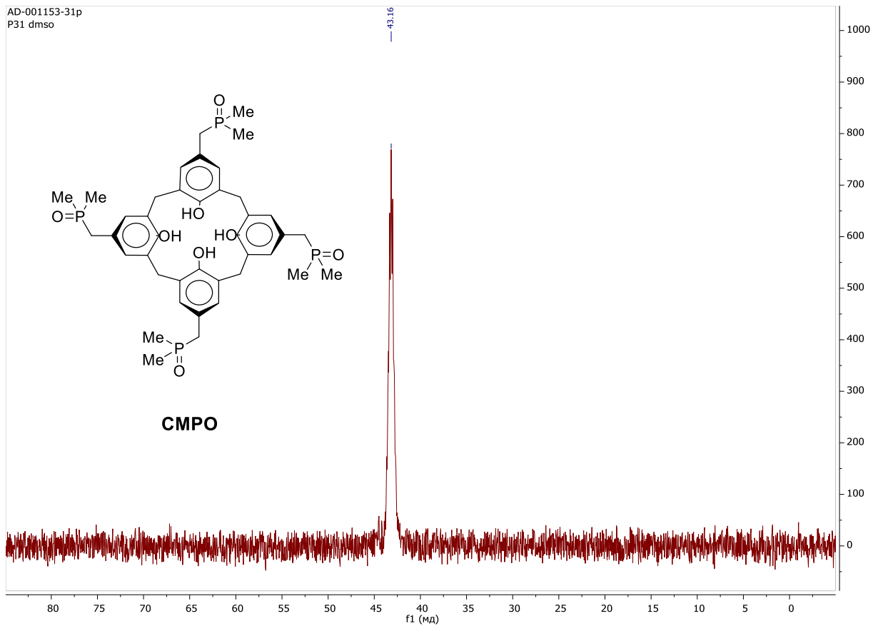
Figure S3. ^{31}\text{P} NMR spectrum of CMPO , (DMSO- d_6 )
