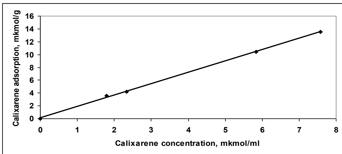
Figure S8. Adsorption isotherm of calixarene TCMPO ( R^2=0.99 ).
