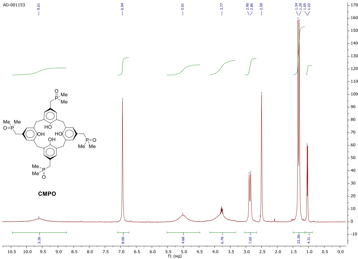
Figure S1. ^1\text{H} NMR spectrum of CMPO , ( \text{DMSO-d}_6 )
