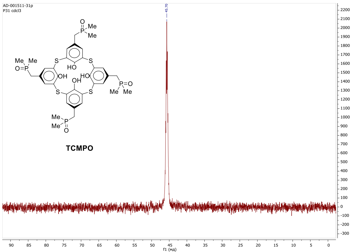
Figure S4. ^{31}\text{P} NMR spectrum of TCMPO , (DMSO- d_6 )
