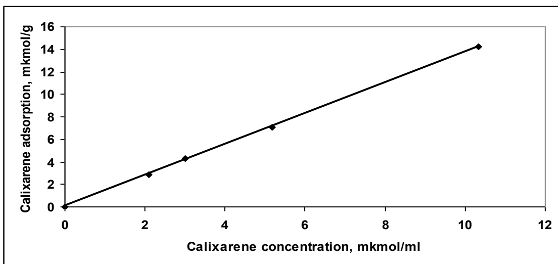
Figure S7. Adsorption isotherm of calixarene CMPO ( R^2=0.99 ).
