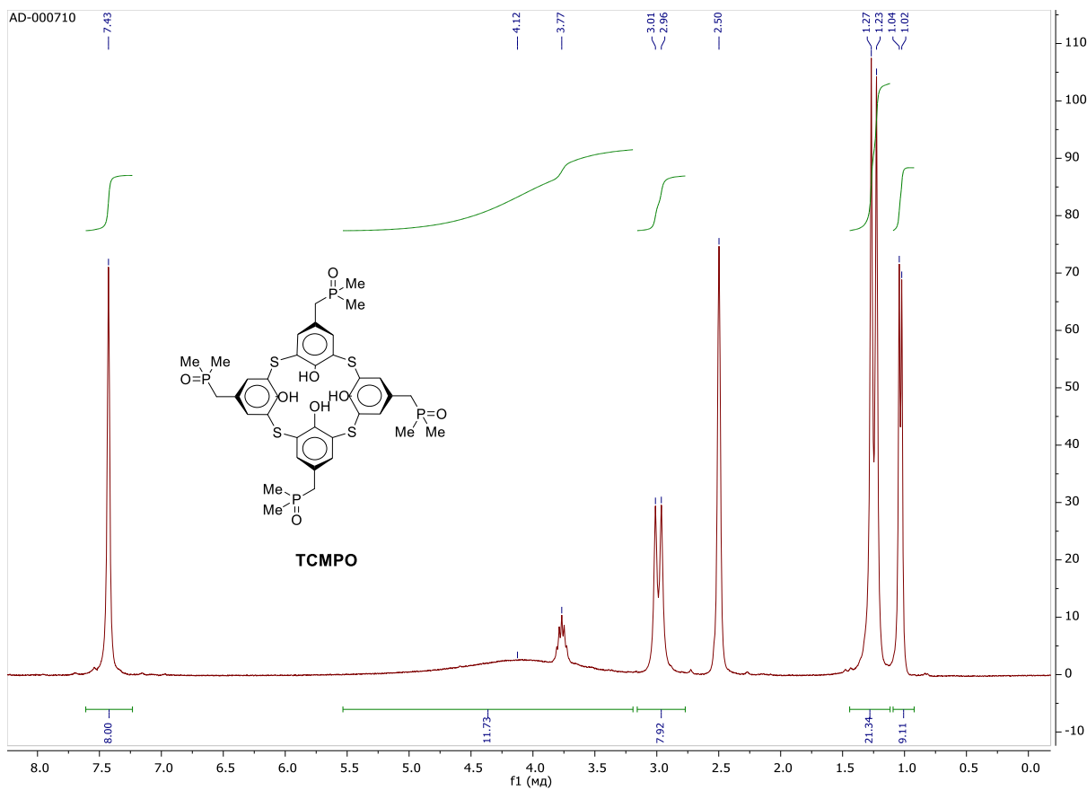
Figure S2. ^1\text{H} NMR spectrum of TCMPO , ( \text{DMSO-d}_6 )
