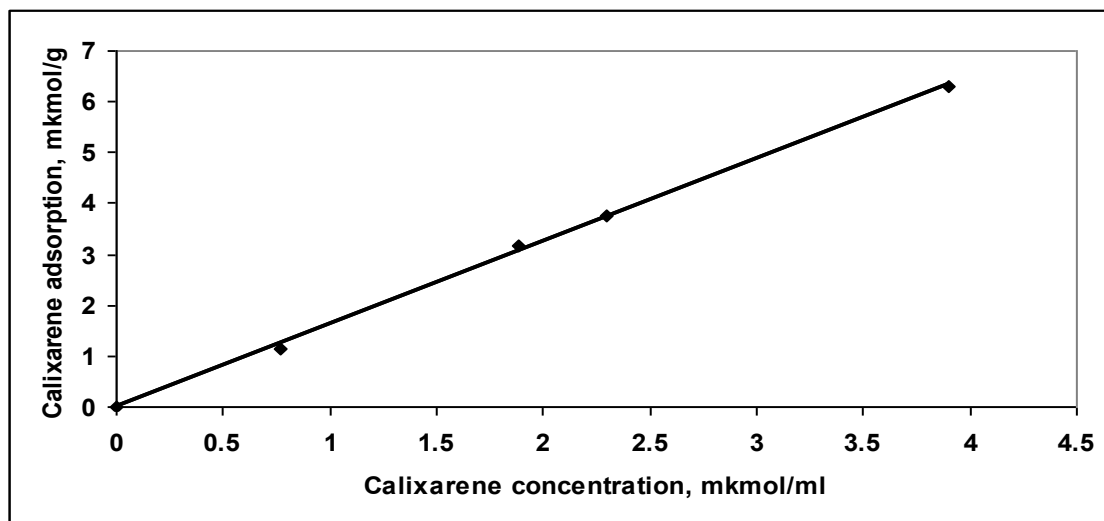
Figure S9. Adsorption isotherm of calixarene CEPO ( R^2 = 0.99 )
