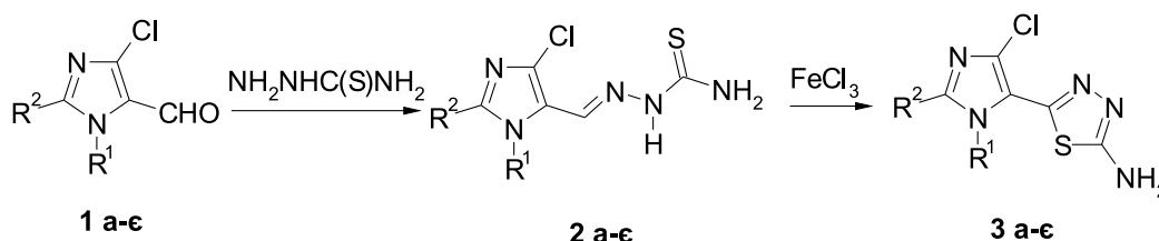
1-3 , R 1 = Ph, R 2 = H (а); R 1 = 4-FC 6 H 4 , R 2 = H (б); R 1 = 4-MeC 6 H 4 , R 2 = H (в); R 1 = Me, R 2 = 3-NO 2 C 6 H 4 (г); R 1 = 4-FC 6 H 4 , R 2 = Cl (д); R 1 = 4-ClC 6 H 4 , R 2 = Cl (е); R 1 = 4-MeC 6 H 4 , R 2 = Cl (е)
