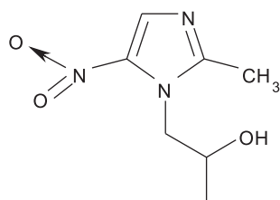
Fig. 1. The chemical structure of secnidazole
